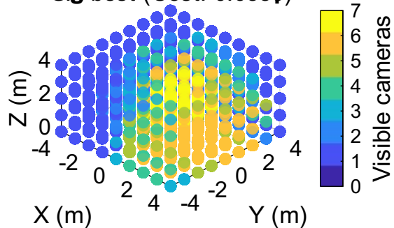
UAV coverage: GA-best vs OptiTrack ad-hoc (Uniform spc = 1.00 m)
